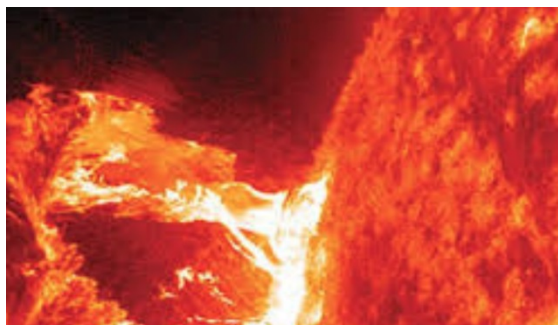
Solar Flare Captured by NASA
