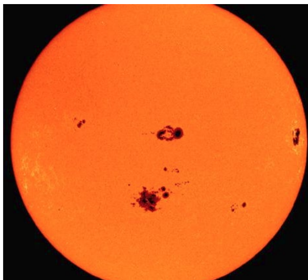
Sunspots
